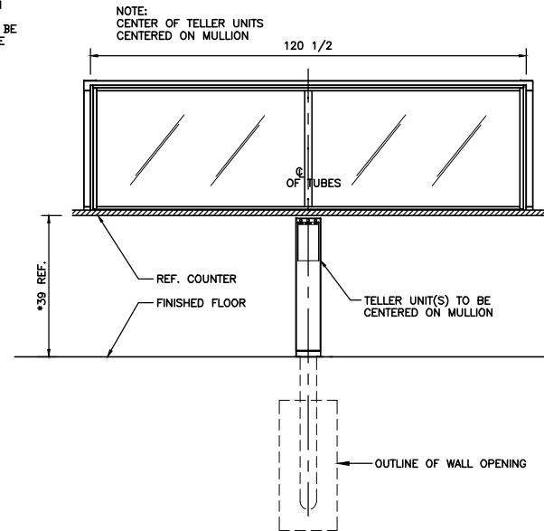
INSIDE ELEVATION
