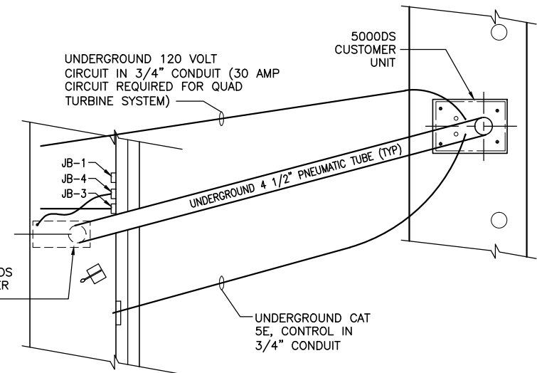
TYPICAL ELECTRICAL LAYOUT
