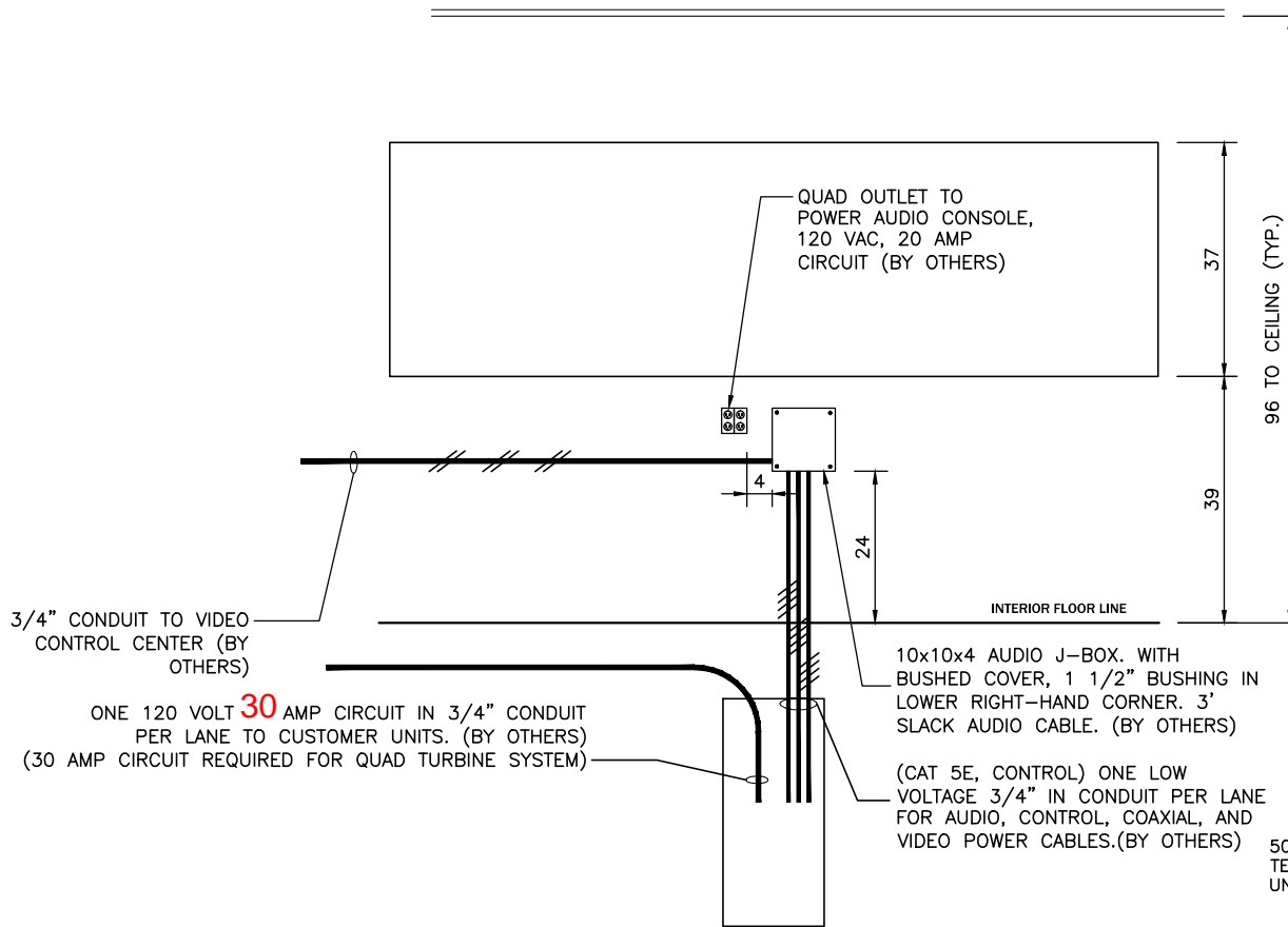
WALL OPENING AND ELECTRICAL DETAIL
