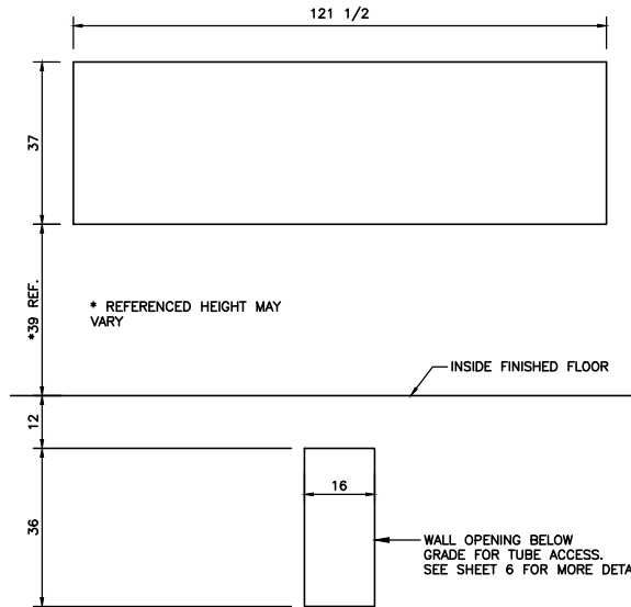
INSIDE ELEVATION MASONRY OPENING
