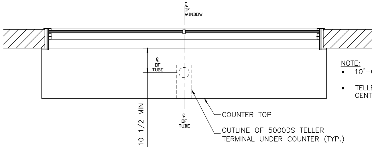
INSIDE PLAN VIEW AT DRIVE-UP COUNTER
