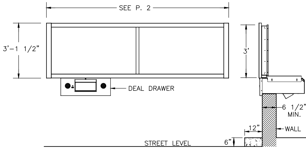
OUTSIDE ELEVATION
