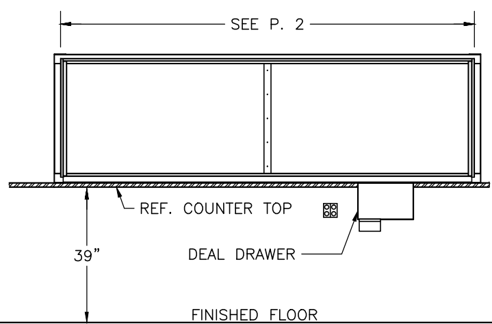
INSIDE ELEVATION
