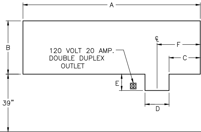
INSIDE ELEVATION MASONRY OPENING
